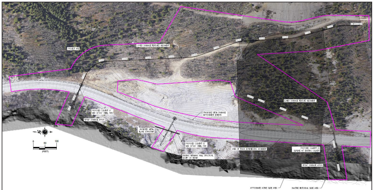
Slope stabilization plans at MP 357.1 include new culverts on the lower slope and fortified ditches on the upper slope.
