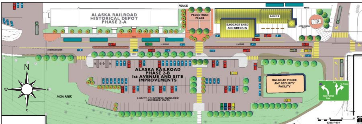
Phase 2b includes parking lot, baggage and check-in area, pedestrian plaza and crew facility. It is not funded.
