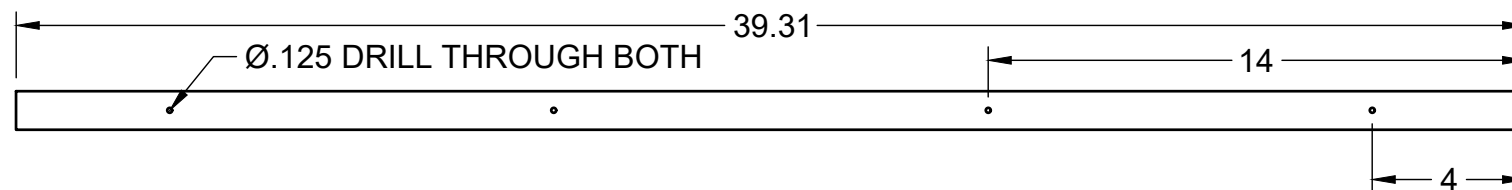
ITEM 10 - ROTATED SIDE VIEW
