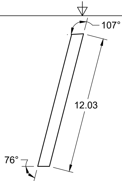
ITEM 3 - TOP VIEW
