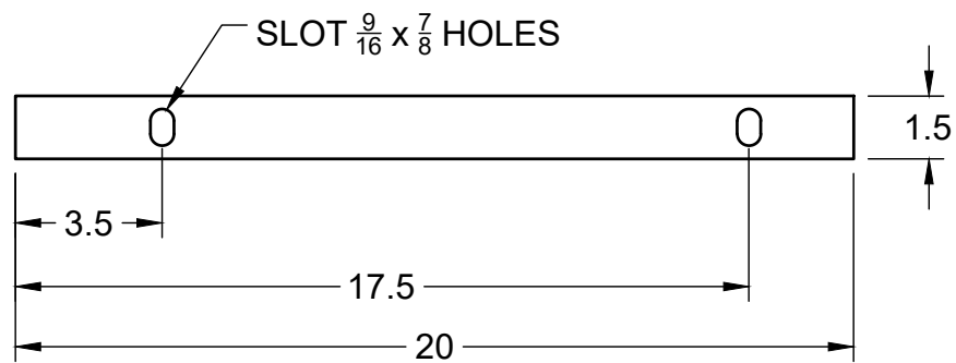
ITEM 2 - TOP VIEW
