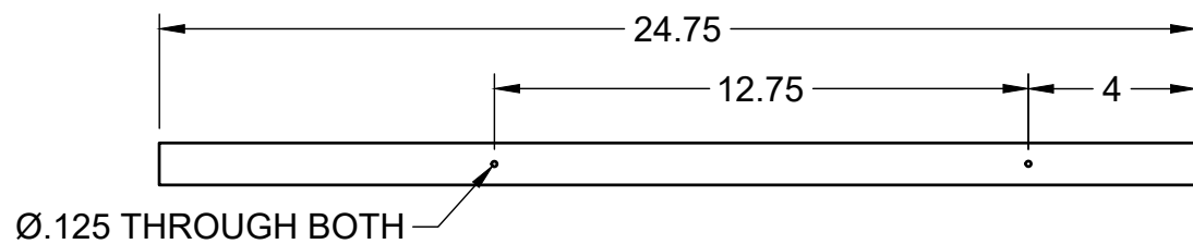
ITEM 11 - ROTATED SIDE VIEW
