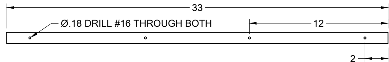
ITEM 12 - TOP VIEW
