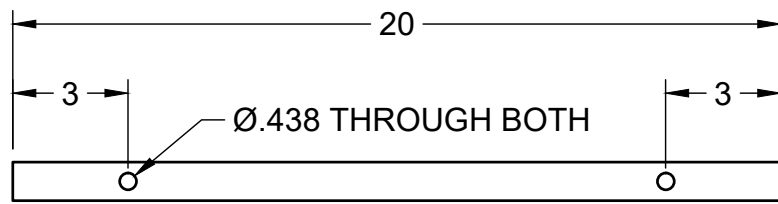
ITEM 3 - TOP VIEW
