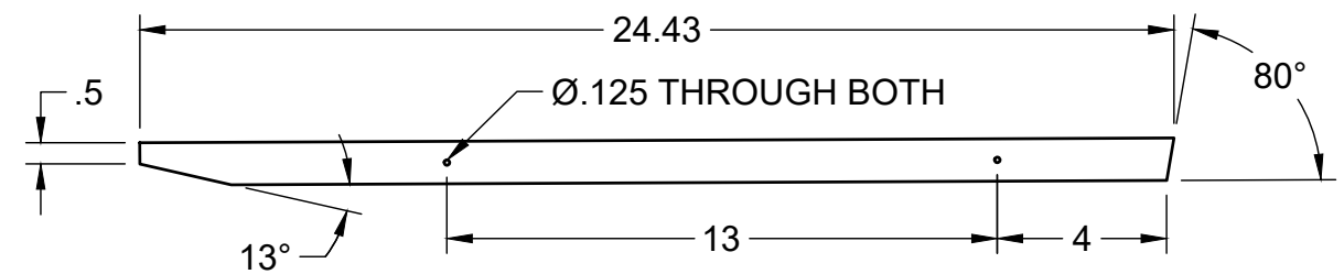
ITEM 9 - ROTATED SIDE VIEW
