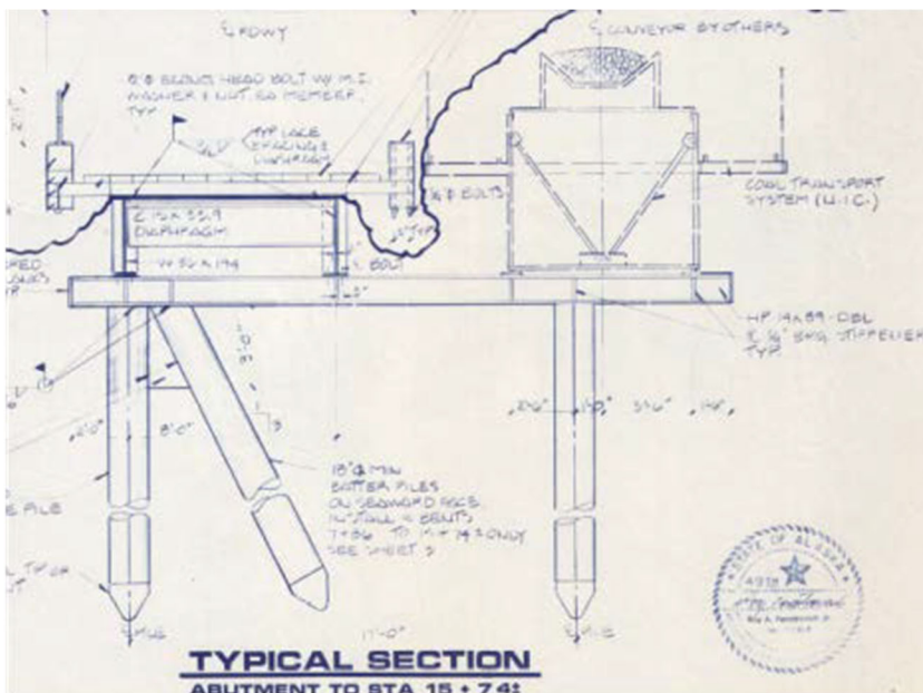
PIER TYPICAL SECTION
