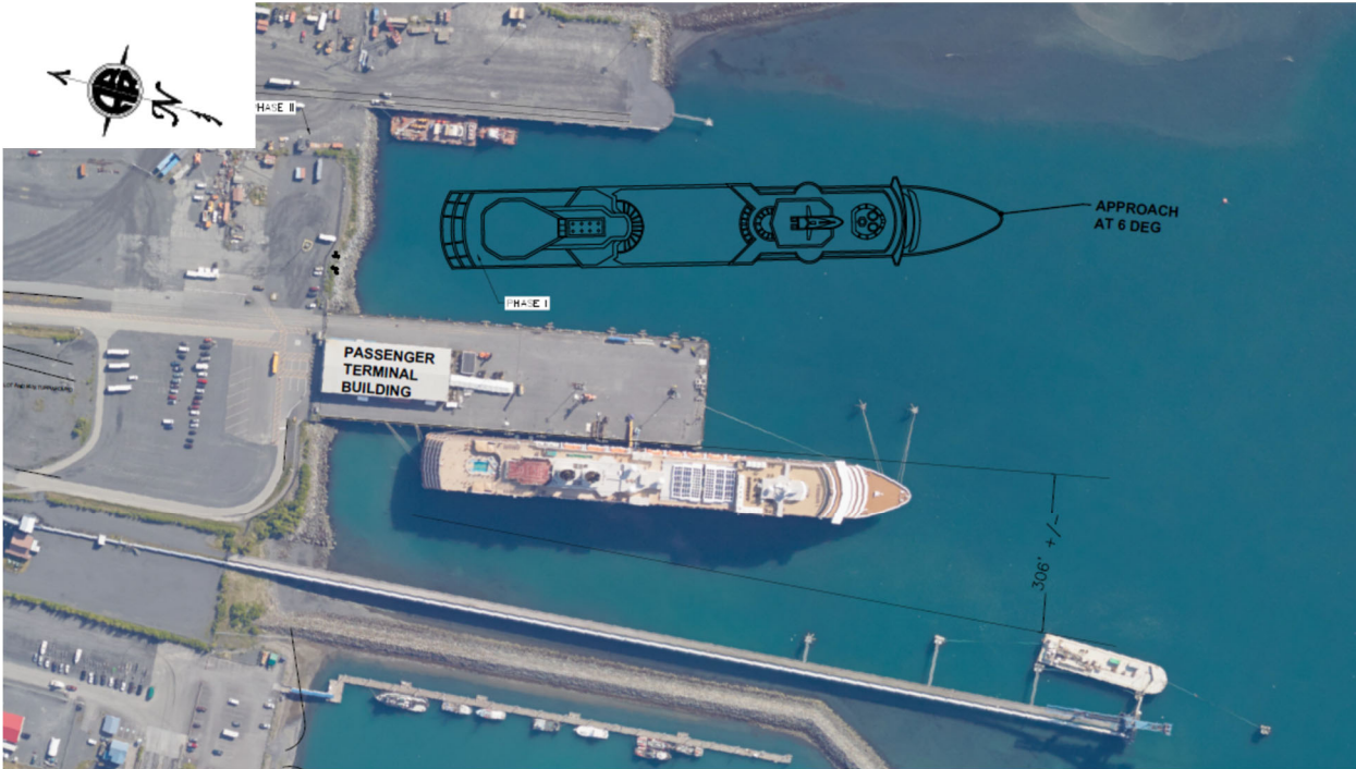
Ship Approach Example
