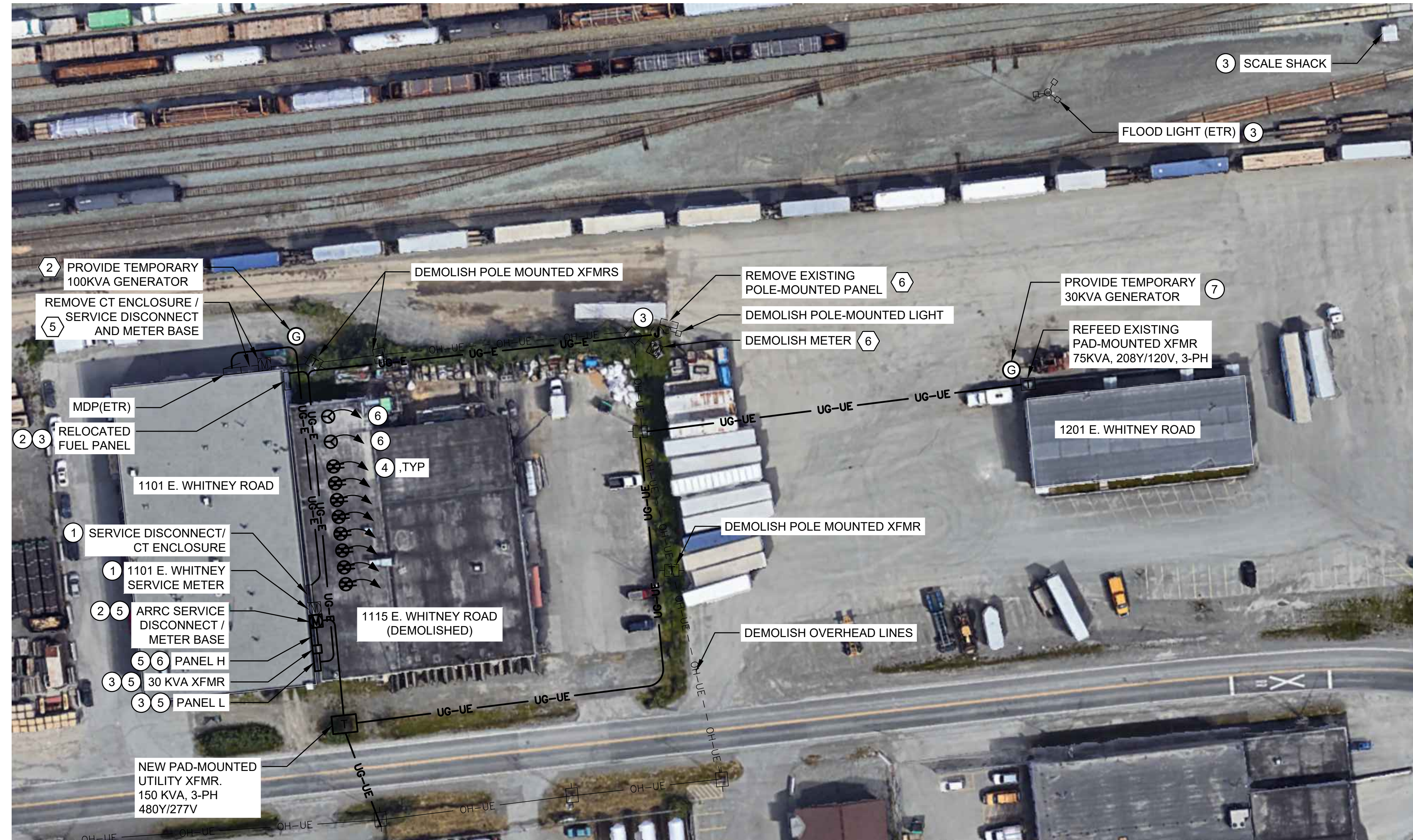
1 ELECTRICAL SITE PLAN E001 1" = 40'-0"
