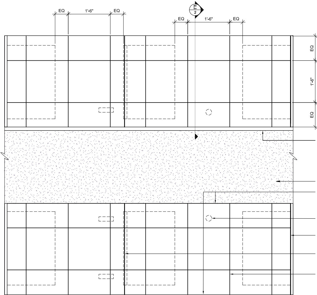
D 2 NO SCALE DETAIL - LOWER LEVEL DINING FLOOR FINISH
