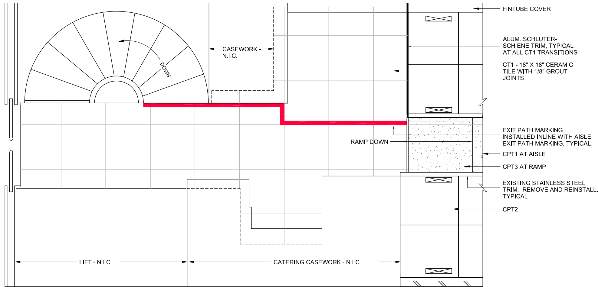
DETAIL - UPPER LEVEL BAR AREA FLOORING NO SCALE
